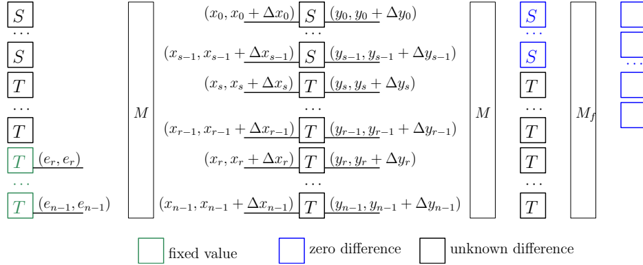
Figure 5: Collision attacks on 3-round Tip5, Tip4 and Tip4' in the fixed-length input case, where the inner part is initialized to 1.
