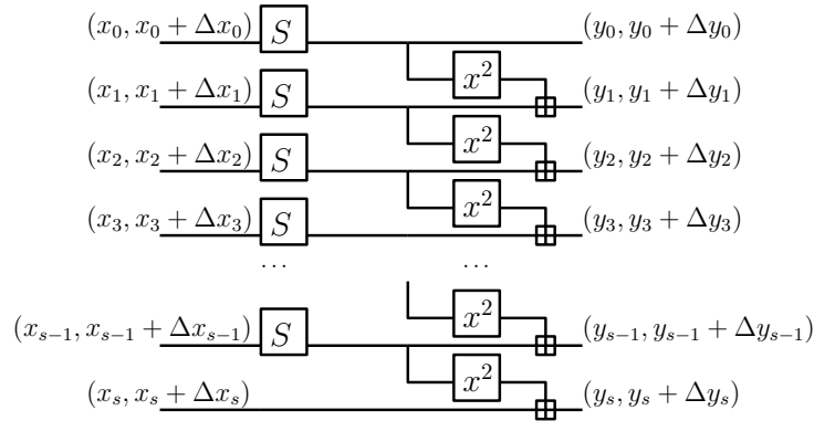
Figure 7: The composition y = \mathcal{F}(\mathcal{B}(x))
