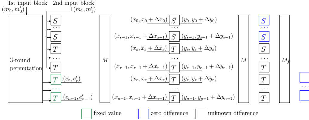
Figure 6: The three-stage 3-round collision attacks, where padding can be ignored.
